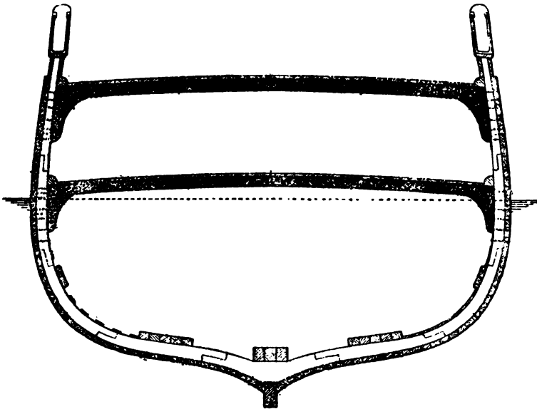
Fig. 335.—Transverse section of a ship. (After Boppe.)
